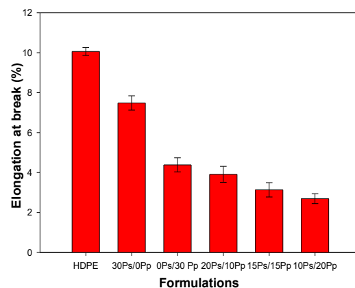
Fig. 3. Evolution of the elongation to rupture of developed composites
