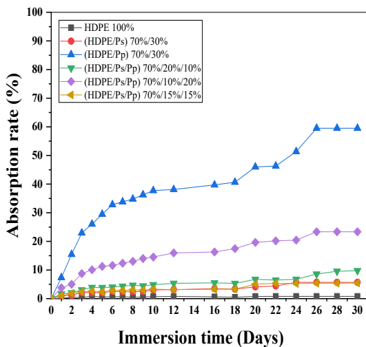
Fig. 7. The evolution of the water absorption rate of the composites developed
