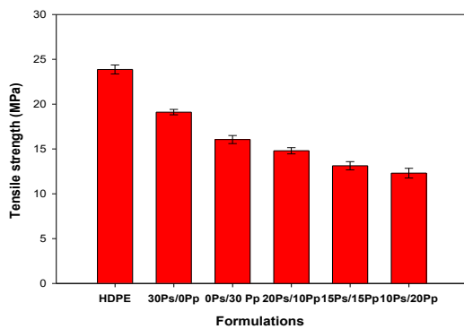
Fig. 1. Evolution of the tensile strength of different formulations
