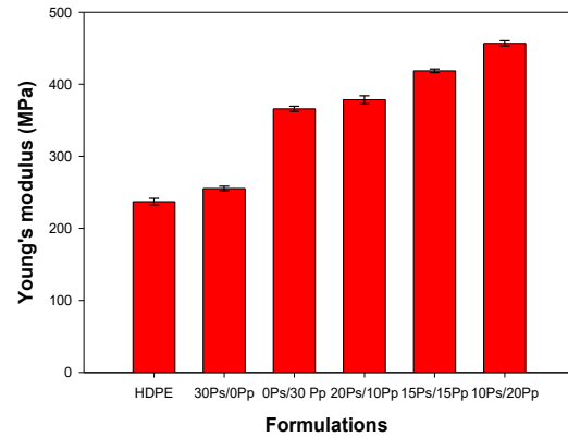
Fig. 2. The evolution of Young's modulus of the developed composites
