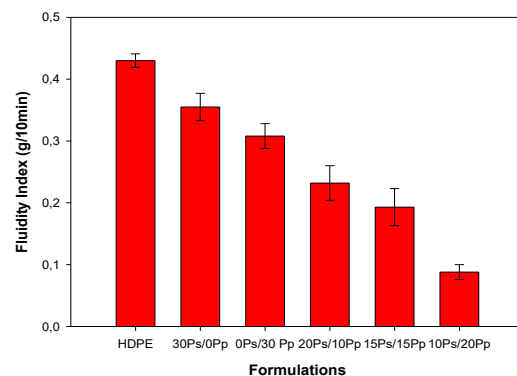
Fig. 6. The evolution of the flow index of the developed composites
