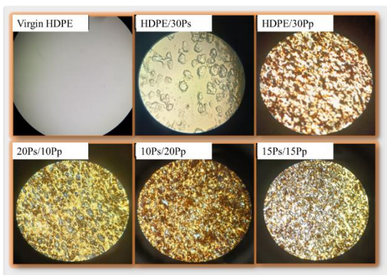
Fig. 9. Optical microscope imaging of the surfaces of the developed composites and virgin HDPE
