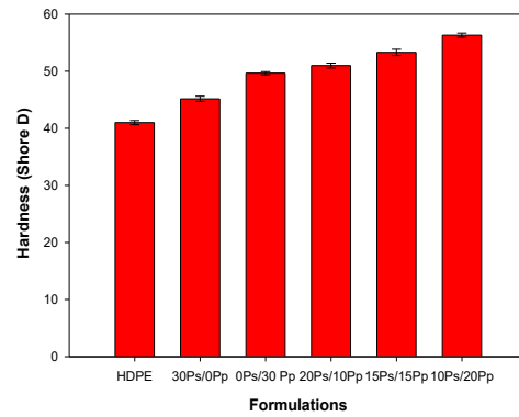
Fig. 5. Evolution of the Shore D hardness of the developed composites
