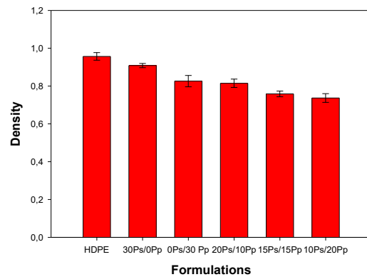
Fig. 8. The evolution of the density of the developed composites
