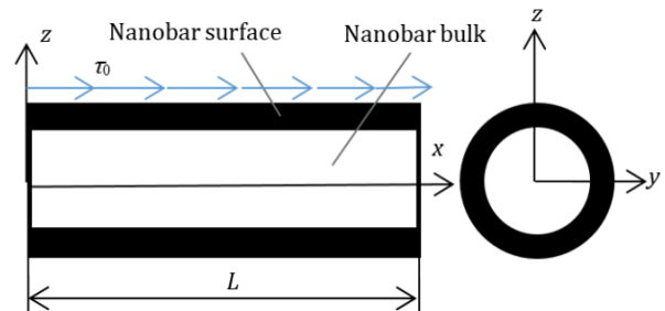
Fig. 1. Schematic of a nanobar with its surface.
