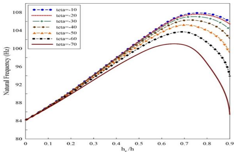
Fig. 9. Influence of Core Thickness and Auxetic Unit Cell Angle on Natural Frequencies in Relatively Thick Shell Structures
