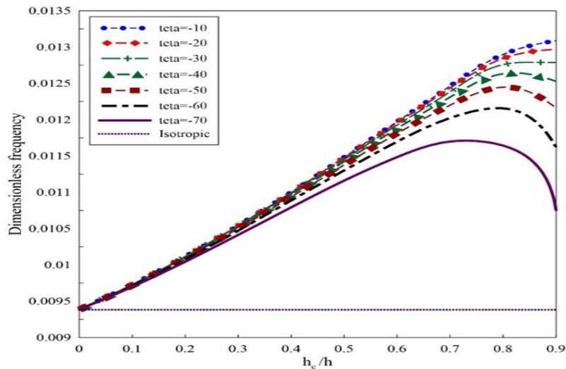
Fig. 8. Effect of Thin Shell Core Thickness and Auxetic Unit Cell Angle on Natural Frequencies
