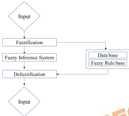
Fig. 3. Fuzzy model for Mechanical strength parameters
