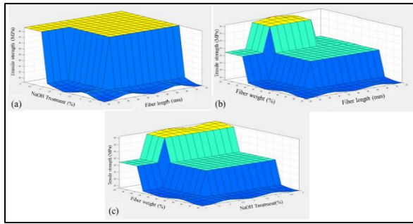
Fig. 8. Surface view plots for tensile strength (a) NaOH treatment vs Fiber length, (b) Fiber weight vs Fiber length, and (c) Fiber weight vs NaOH treatment
