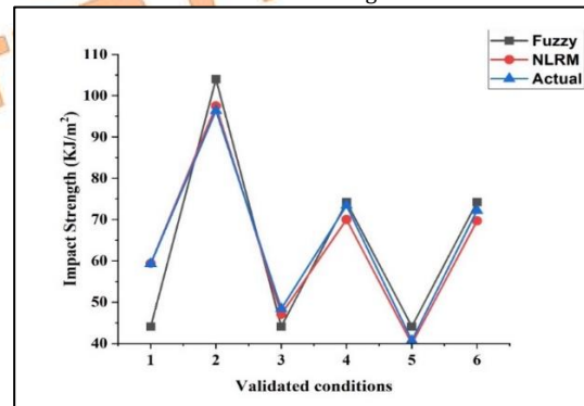
Fig. 13. Comparison of experimental and predicted values of Impact strength
