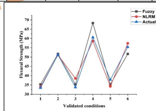
Fig. 12. Comparison of experimental and predicted values of Flexural strength
