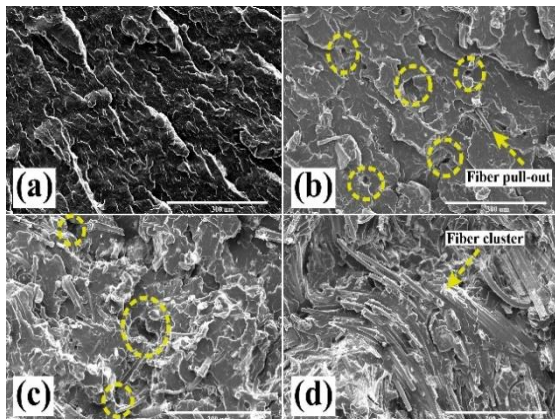
Fig. 2. SEM images of (a) Polypropylene, (b) 15 wt.% of hemp fibers-reinforced polypropylene composite, (c) 30 wt.% of hemp fibers-reinforced polypropylene composite, (d) 45 wt.% of hemp fibers-reinforced polypropylene composite
