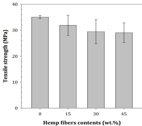
Fig. 5. Tensile strength of polypropylene and their hemp fibers-reinforced composites with different fiber contents
