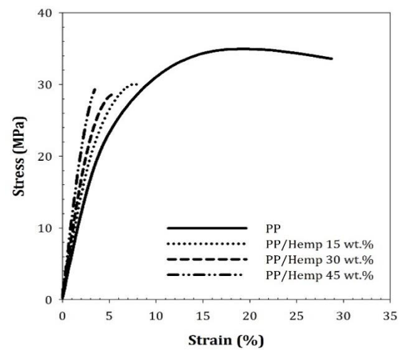
Fig. 3. Tensile stress-strain curves of polypropylene and their hemp fibers-reinforced composites
