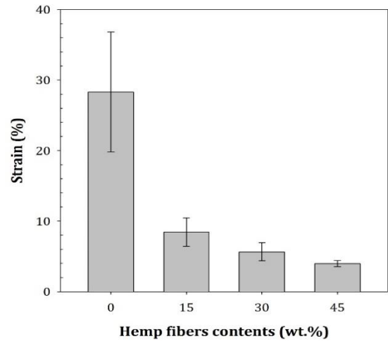
Fig. 6. Strains at break of polypropylene and their hemp fibers-reinforced composites with different fiber contents
