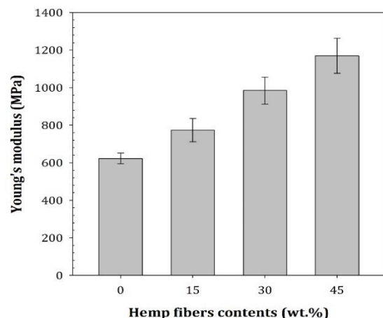
Fig. 4. Young's modulus of polypropylene and their hemp fibers-reinforced composites with different fiber contents
