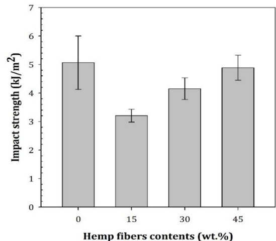
Fig. 7. Impact strength of polypropylene and their hemp fibers-reinforced composites with different fiber contents.
