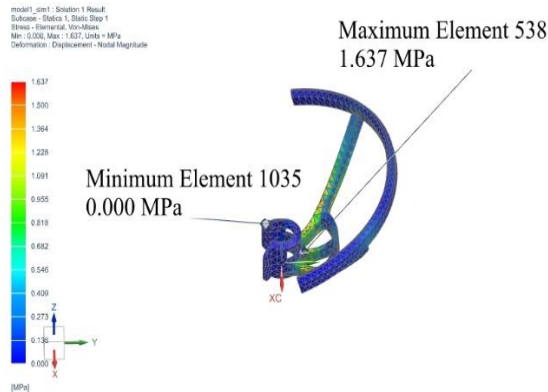
Fig. 8. Stress distribution of DJI Tello propeller guard derived from SIMCENTER 3D simulation
