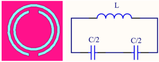
Fig. 2. Equivalent circuit of CSRR
