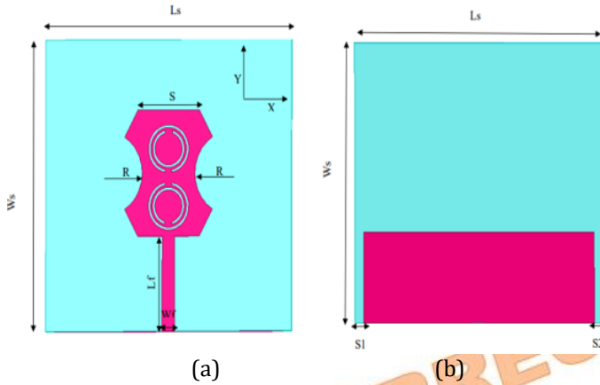
Fig. 5. Layout of Proposed Antenna (a) top view (b) bottom view
