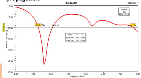
Fig. 11. Bandwidth plot of proposed antenna at -10 dB
