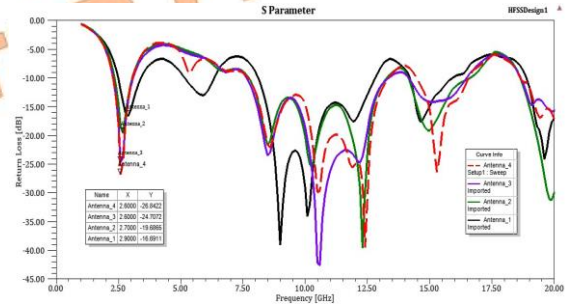
Fig. 7. S-Parameter for Evolution Of Proposed Antenna
