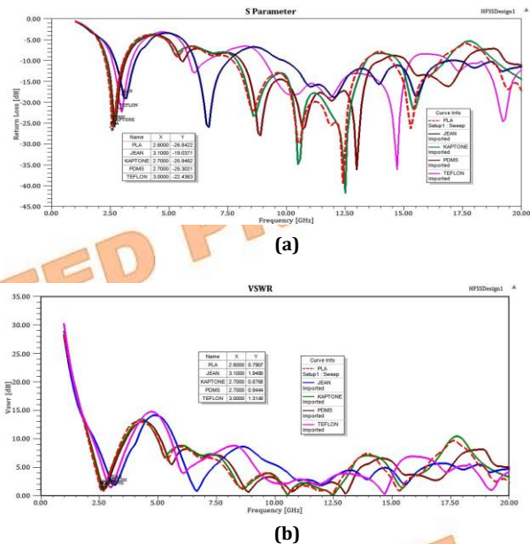
Fig. 6. S-Parameter (a) & VSWR (b) for PLA and Various Substrates
