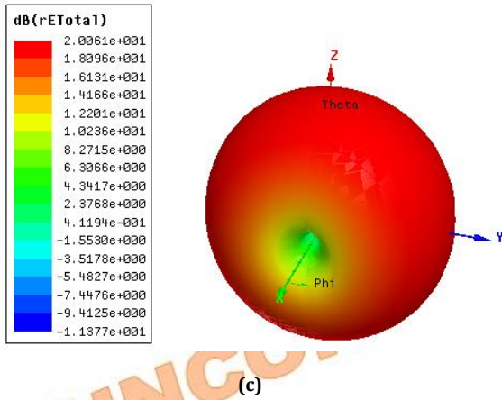
Fig. 9. E & H planes (a), (b), and 3D plot (c) of Radiation Pattern
