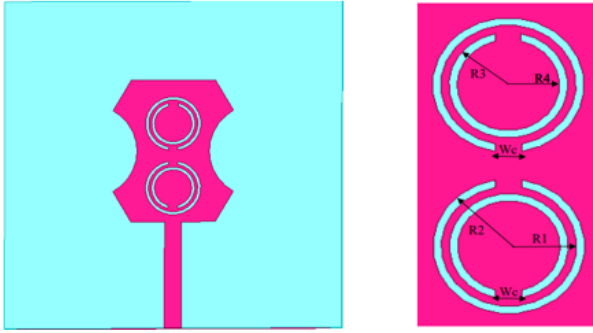
Fig. 1. Layout of Proposed Antenna with CSRR
