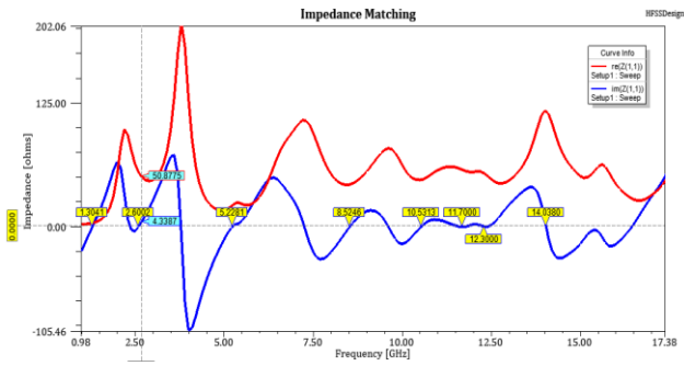
Fig. 14. Impedance plot of proposed antenna for 2.6 GHz Impedance matching is a crucial aspect of antenna design, ensuring efficient power transfer between the transmission line and the antenna itself. Achieving impedance matching is essential for minimizing signal loss and maximizing the effectiveness of the antenna system in various communication applications. In the analysis, the proposed antenna achieved a 50-ohm impedance represented in Fig. 14, which signifies a successful impedance match, as it corresponds to the standard impedance commonly used in radio frequency systems. This alignment ensures optimal power transfer between the antenna and the transmission line, indicating that the antenna is well-matched to the [26]desired impedance specifications.
