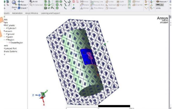
Fig. 16. Conformal analysis for the proposed wearable antenna
