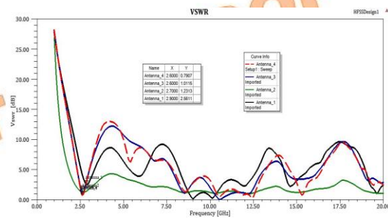
Fig. 8. VSWR for Evolution Of Proposed Antenna
