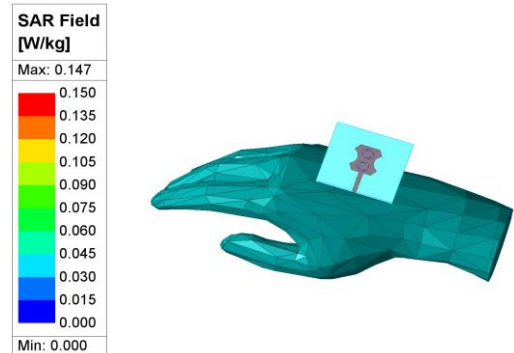
Fig. 15. SAR analysis for the proposed wearable antenna at 2.6 GHz
