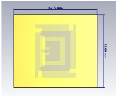
Fig. 2. Substrate dimension
