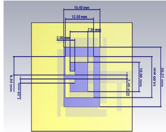
Fig. 5. Dimensions of parasitic patch
