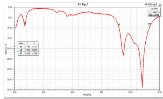
Fig. 15. Return loss for an active patch with slots
