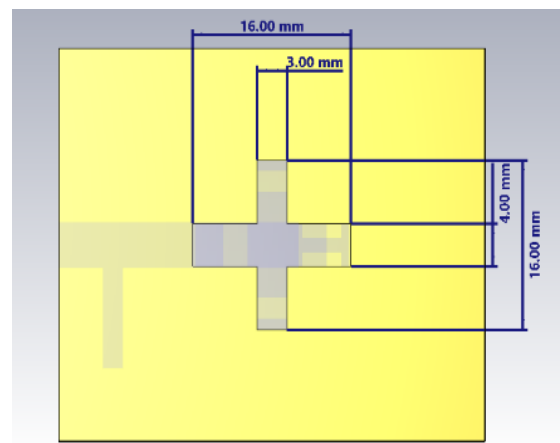
Fig. 6. Dimensions of the ground plane with "+" slot
