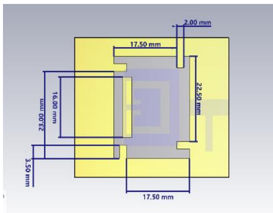
Fig. 4. Dimensions of active patch
