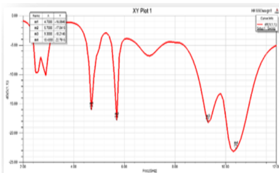
Fig. 14. Return loss for "+" slot in ground plane
