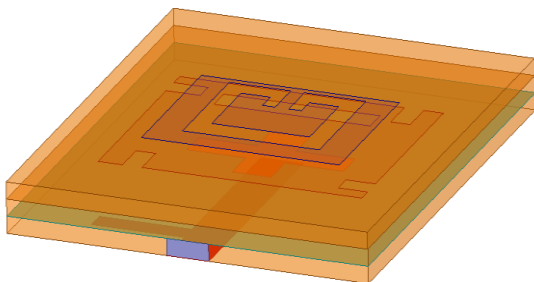
Fig. 9. Final antenna structure with the different stacked layers
