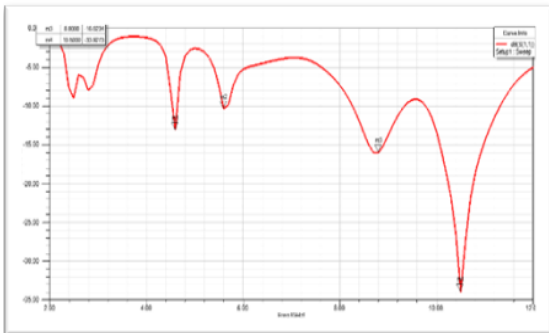
Fig. 13. Return loss for a vertical slot in the ground plane
