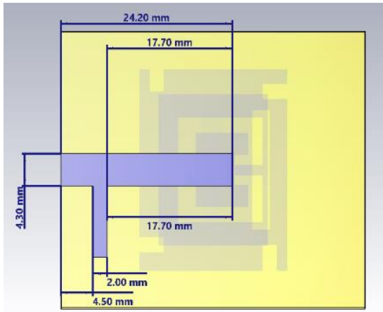
Fig. 7. Dimensions of feedline with stub
