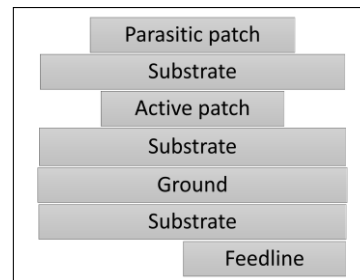
Fig. 1. Geometry of three-layer stacked microstrip patch antenna
