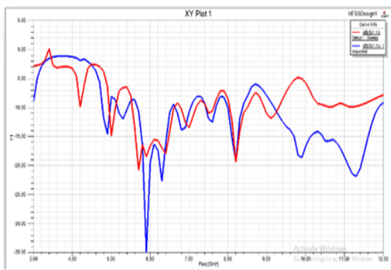
Fig. 19. Results comparisons of feed stub
