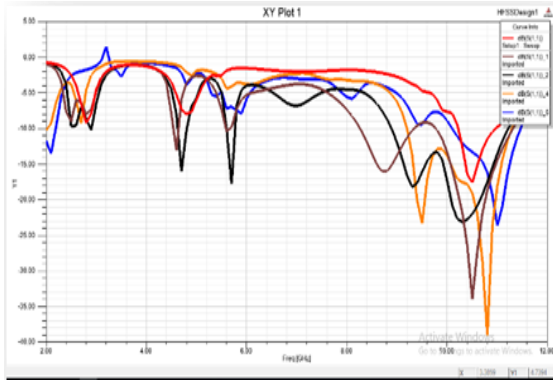
Fig. 17. Results comparisons of ground slots
