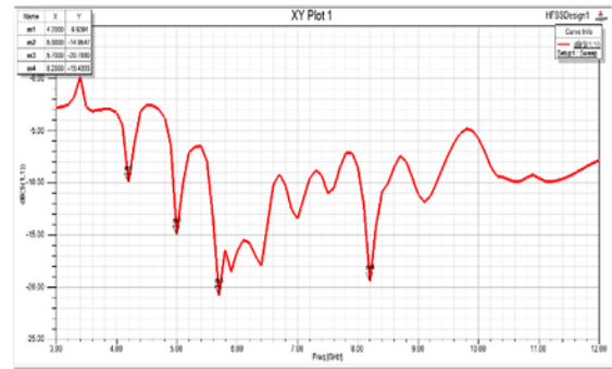
Fig. 16. Return loss for a parasitic patch with slots
