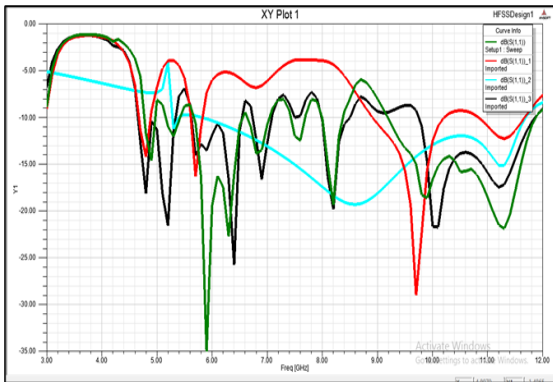
Fig. 18. Results comparisons of patch slots
