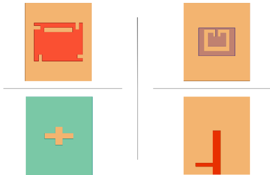
Fig. 8. Different layers of the designed antenna
