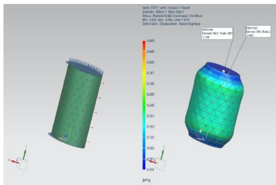
Fig. 7. The stress distribution results for a tank designed to withstand a maximum pressure of 13,300 N/m 2
