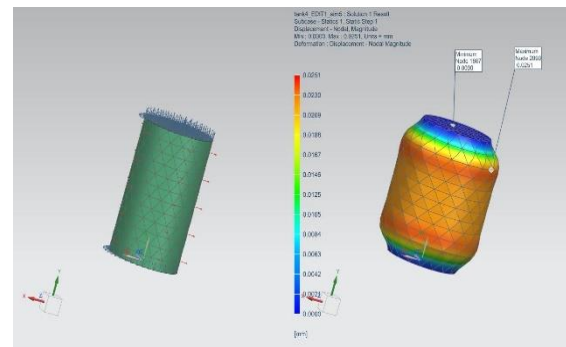
Fig. 8. The deformation results for a tank designed to withstand a maximum pressure of 13,300 N/m 2
