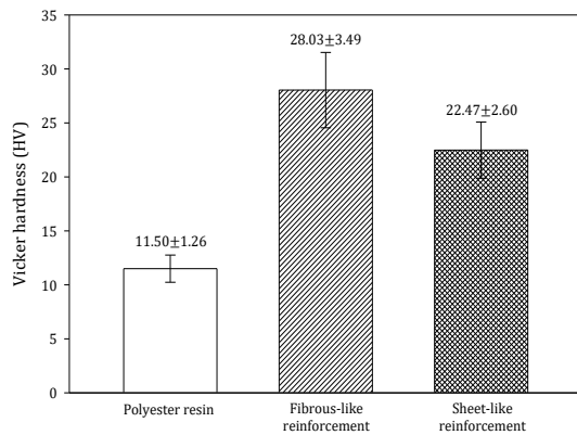
Fig. 3. Hardness of glass fiber-reinforced polyester resin composite
