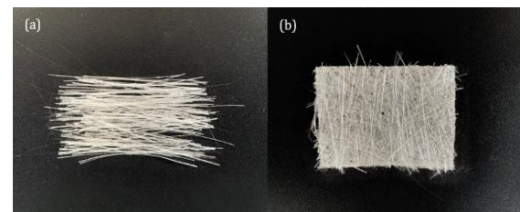
Fig. 1. Glass fibers in two different architectures: (a) fibrous-like and (b) sheet-like.
