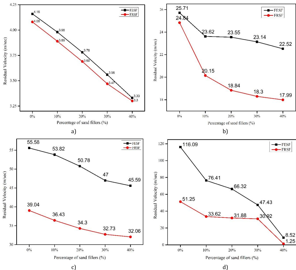
Fig. 5. Residual Velocity for FESF and FRSF for different Velocity a) Low, (10 m/sec), b) Intermediate (50 m/sec), c) High (100 m/sec) and d) Ballistic (350 m/sec)
