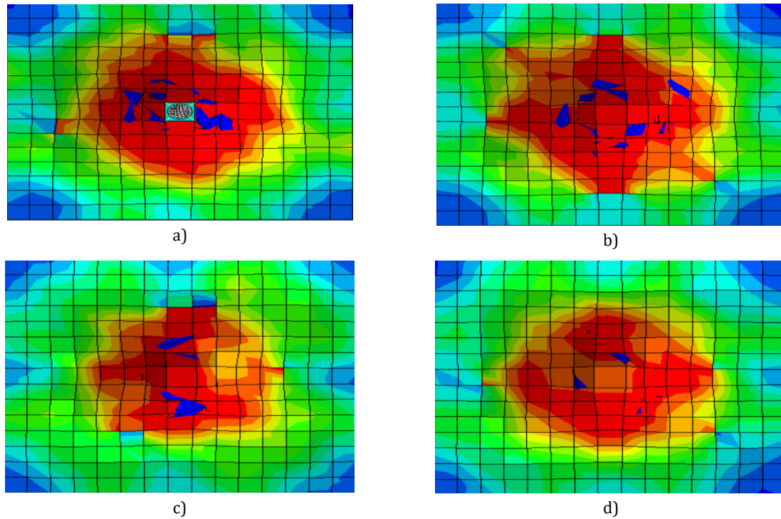
Fig. 10. Damage Behaviour for different core thicknesses in FESF40 a) 5, b) 10, c) 15, and d) 20mm.
