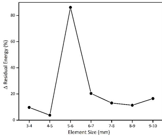
Fig. 3. Mesh convergence for the difference in residual energy % with Element size.
