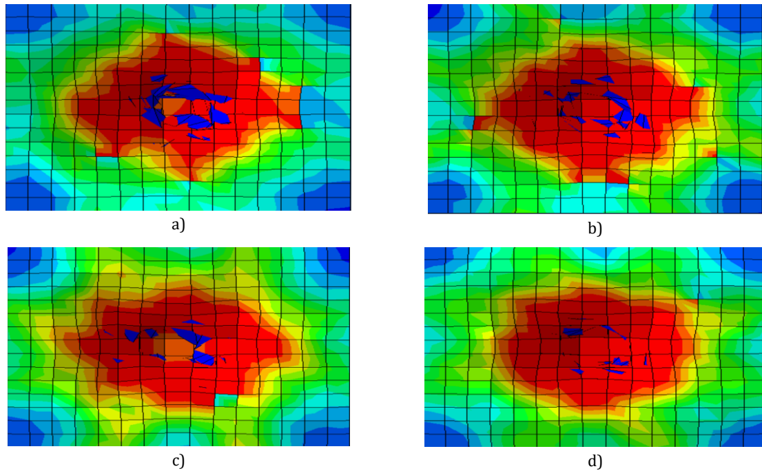
Fig. 11. Damage Behaviour for different core thicknesses in FRSF40 a) 5, b) 10, c) 15 and d) 20mm
