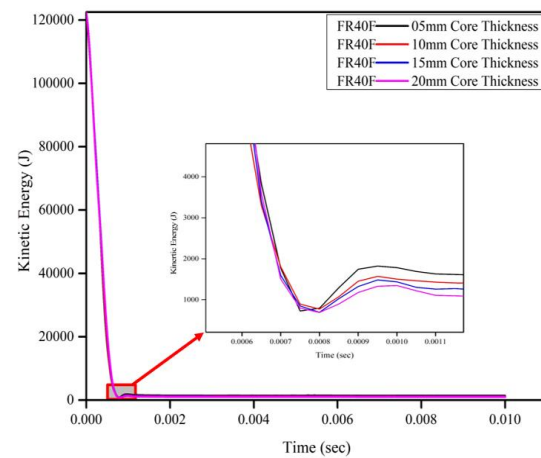
Fig. 7. Variation in Kinetic energy (J) for FR40F
