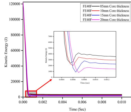
Fig. 6. Variation in Kinetic energy (J) for FE40F
