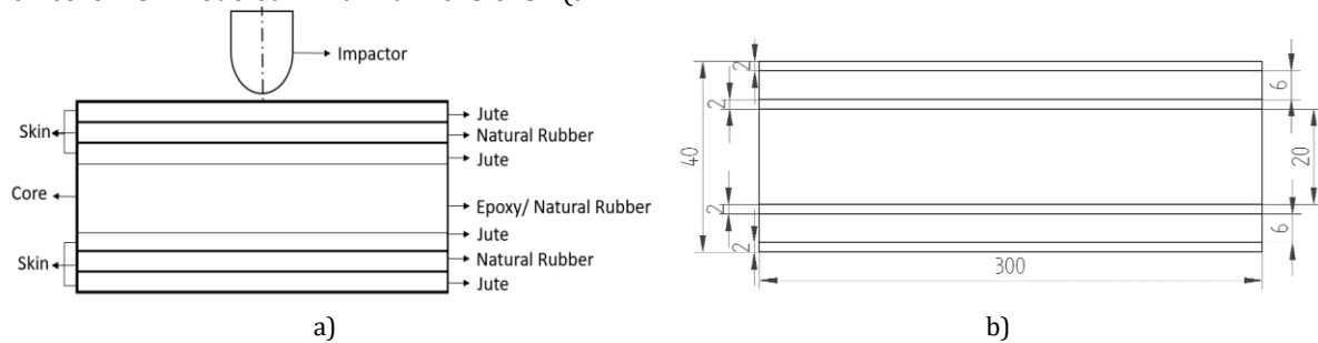
Fig. 1. Sandwich composite subjected to impact a) Sequencing of materials for sandwich structure, b) Dimensioning of sandwich structure (core and skin)
