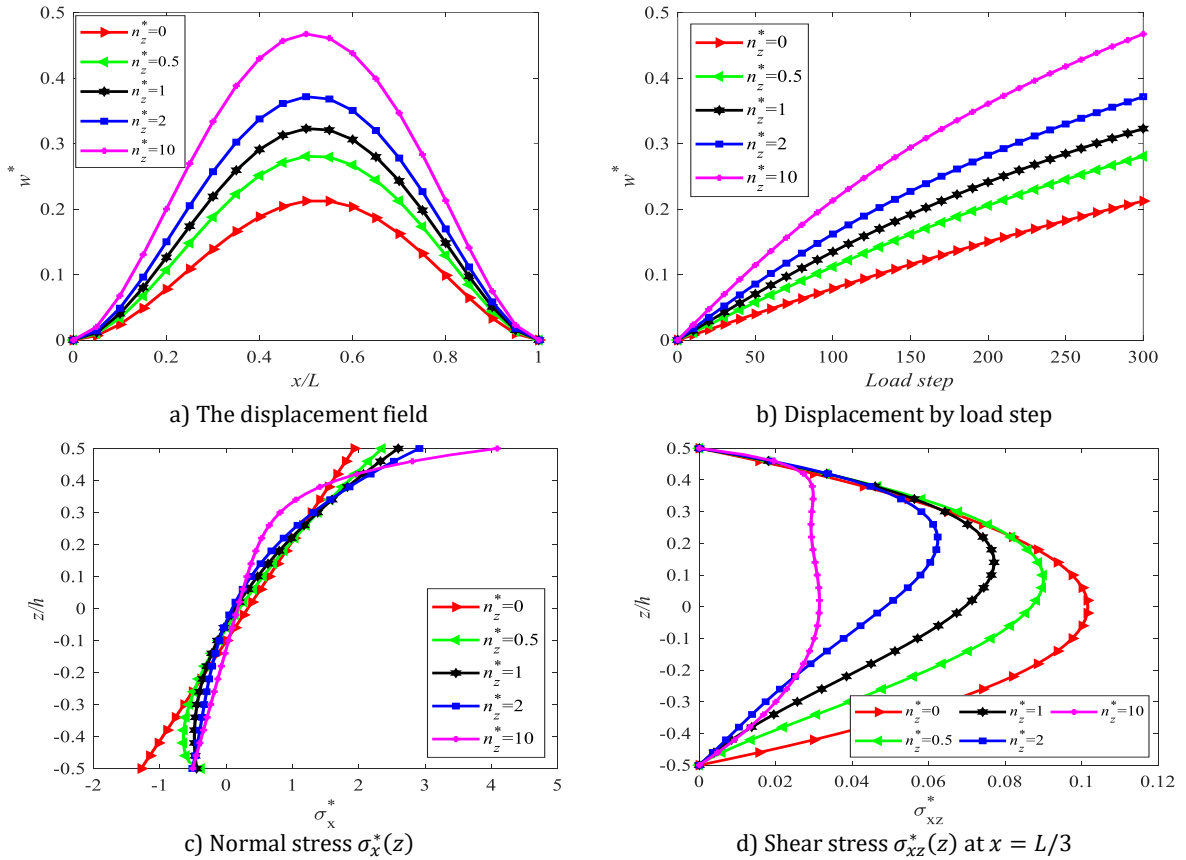
Fig. 8. Effect of the parameter n_z on the nonlinear static response of CC 2DFG-McrBs under SL (Input parameter: \bar{Q} = 300 ; L = 20h ; n_x = 1 ; K_W = 75 ; K_G = 50 ; h^* = 2 )
