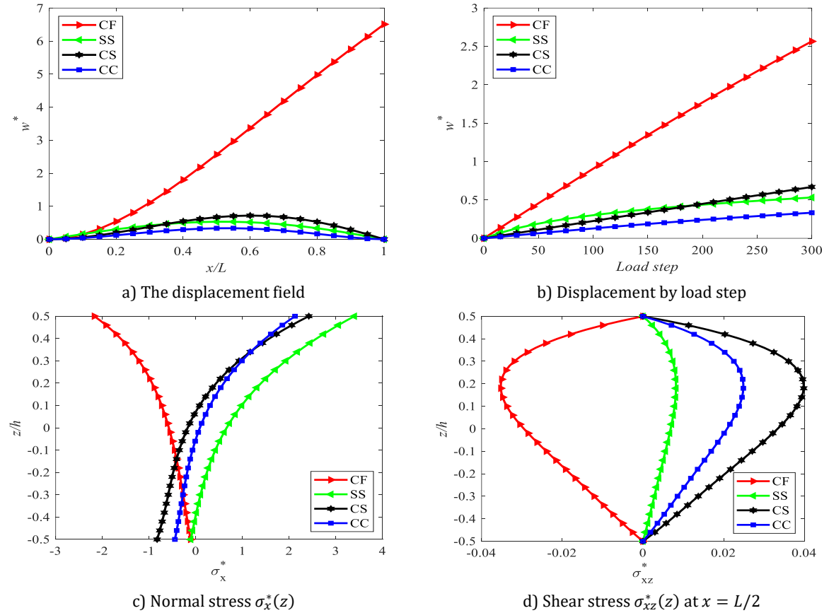
Fig. 10. Effect of BCs on the nonlinear static response of 2DFG-McrBs under UL (Input parameter: \bar{Q} = 300 ; L = 20h ; n_x = n_z = 2 ; K_W = K_G = 25 ; h^* = 1 )
