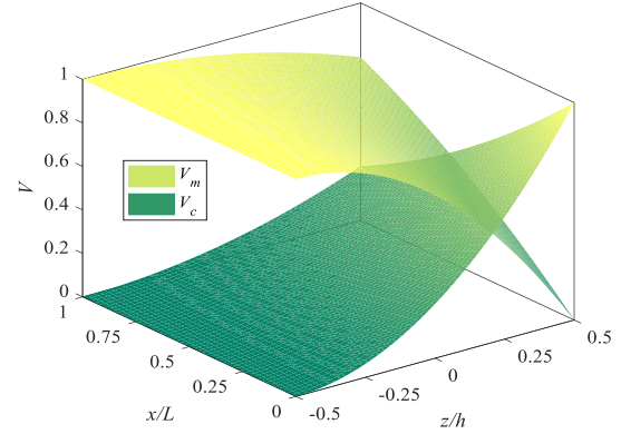
a) The volume fraction of phases
