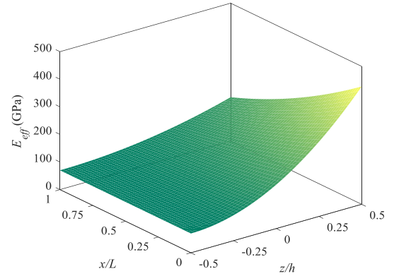
b) The effective elastic modulus
