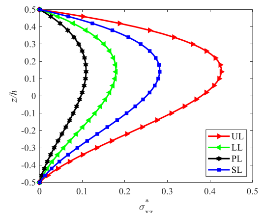
d) Shear stress \sigma_{xz}^*(z)
