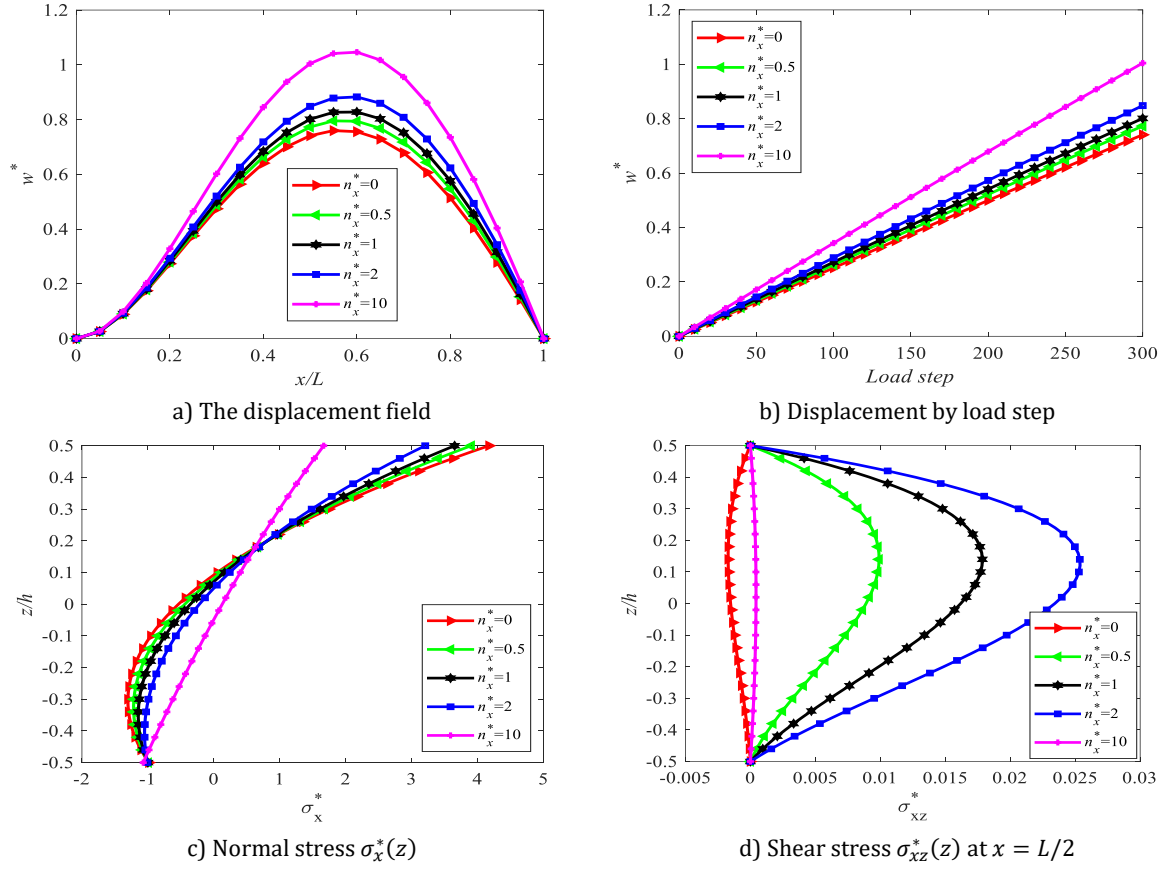
Fig. 9. Effect of the parameter n_x on the nonlinear static response of CS 2DFG-McrBs under UL (Input parameter: \bar{Q} = 300 ; L = 20h ; n_z = 1 ; K_W = K_G = 75 ; h^* = 3 )
