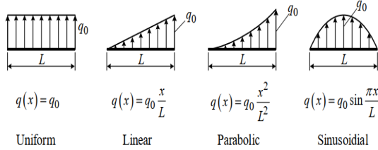
Fig. 2. Various types of loads
