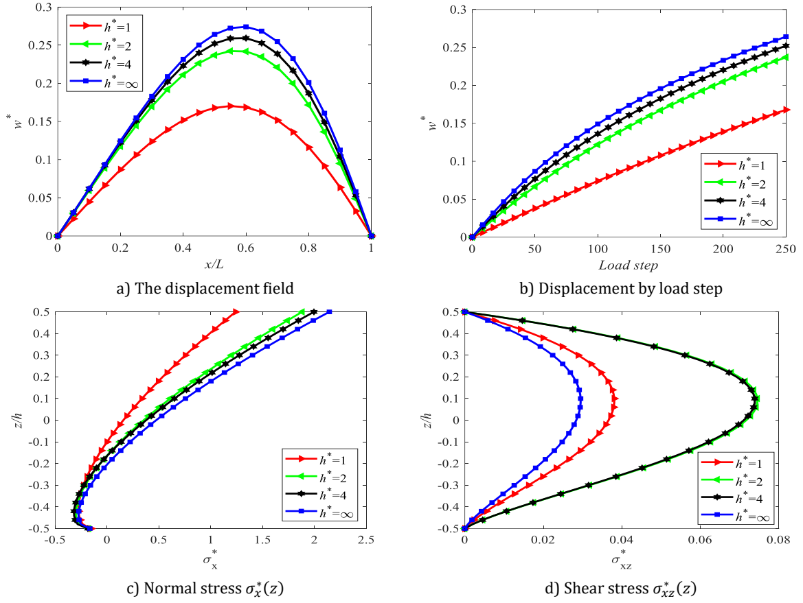
Fig. 7. Effect of the parameter h^* on the nonlinear static response of SS 2DFG-McrBs under PL (Input parameter: \bar{Q} = 250 ; L = 25h ; n_x = n_z = 0.5 ; K_W = K_G = 50 )
