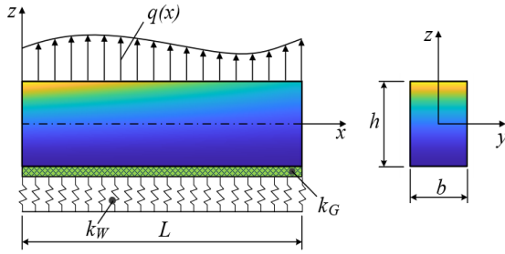
Fig. 1. The 2DFG-McrB model resting on EF
