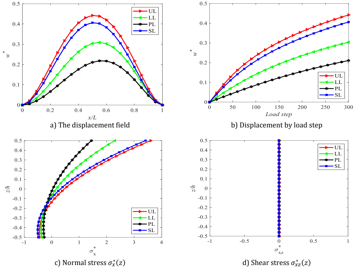
Fig. 5. Effect of load types on the nonlinear static response of CC 2DFG-McrBs
